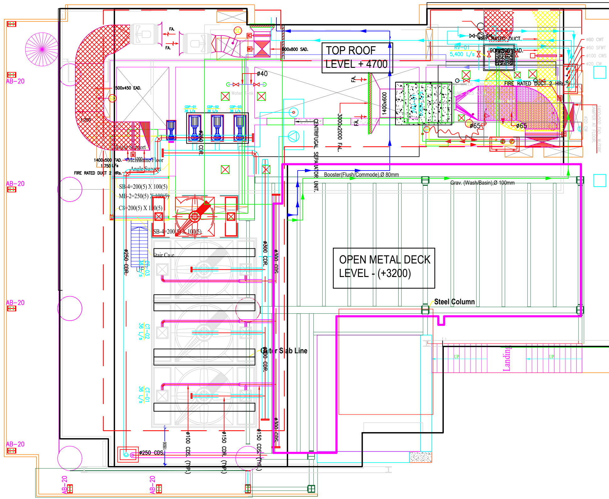
TOP ROOF, METAL DECK
